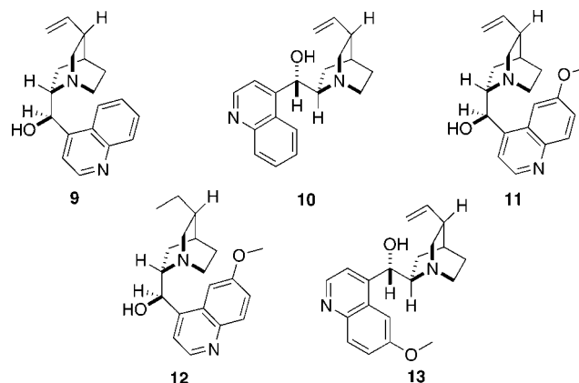
Figure 2. Cinchona alkaloid catalysts.
