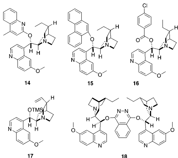
Figure 3. Cinchona alkaloid derivatives.
