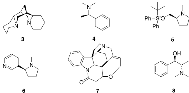
Figure 1. Tertiary amine catalysts.
